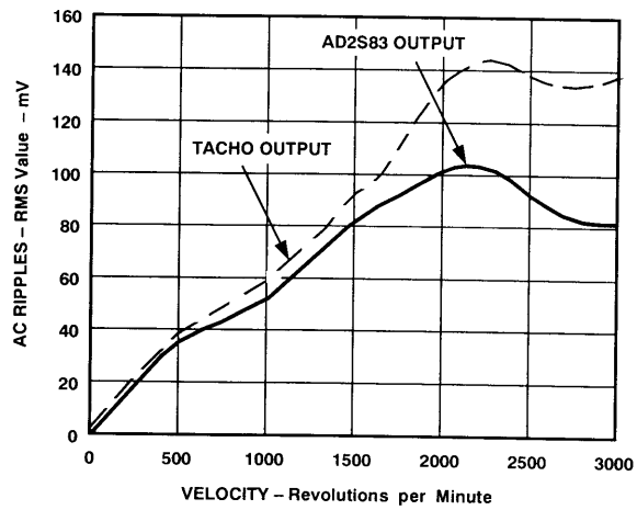
Figure 5. AC Ripple Content Comparison Curve
